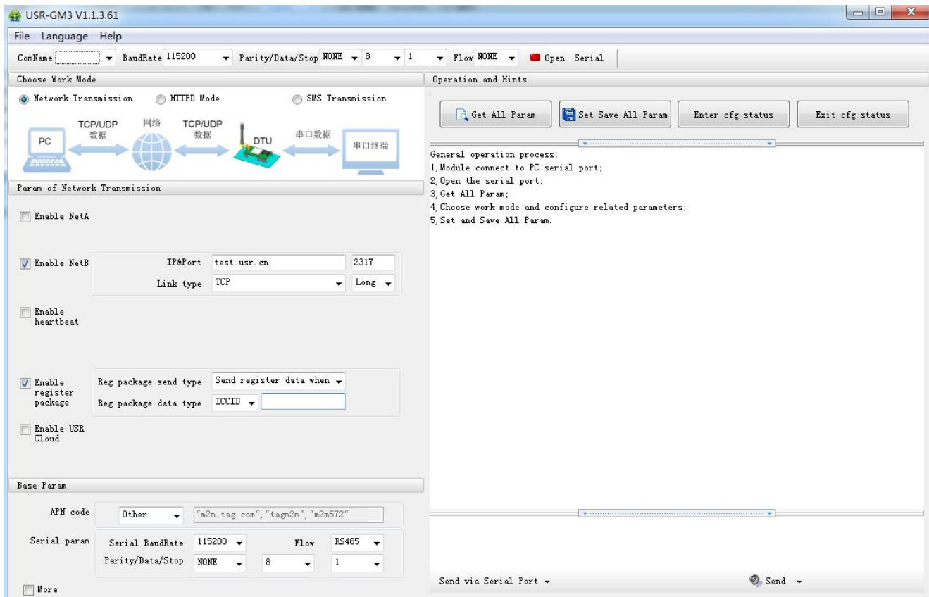
Figure 15 Setup software
